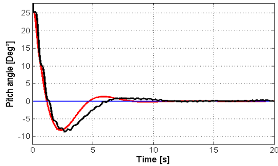
Fig. 14. Simulated and experimental pitch angle step response using the following controllers coefficients ( k_p = 0.3 , k_i = 0.29 , k_d = 0.28 )
