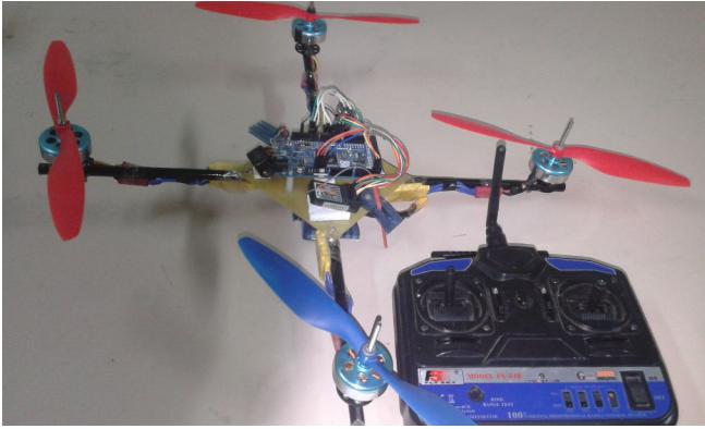
Fig. 3. Sunbird quadrotor prototype
