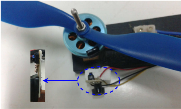
Fig. 6. Infra-Red sensor used for the motor speed measuring
