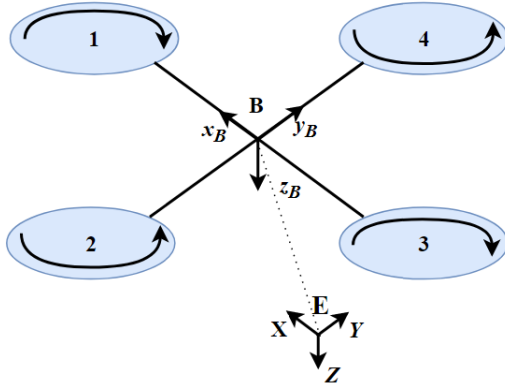
Fig. 1. Quadrotor UAV coordinate system
