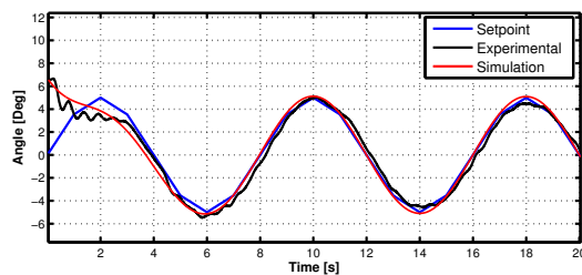
Fig. 16. Tracking of roll sine setpoint simulation and experimental responses
