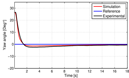
Fig. 15. Yaw angles compared estimated and measured step response with PID controller parameters ( k_p = 0.086 , k_i = 0.006 , k_d = 0.25 )
