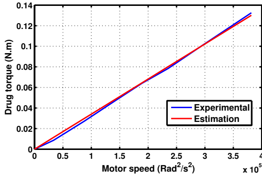
Fig. 11. Measured and approximated of drag moment relative to the square of the motor speed
