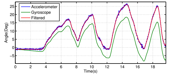
Fig. 4. Comparison of accelerometer ,gyroscope and complementary filter estimated roll angle
