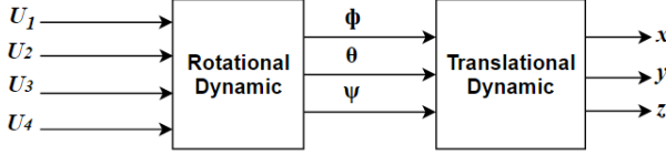
Fig. 2. Quadrotor system architecture
