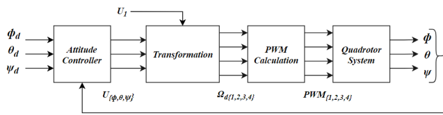
Fig. 12. Control architecture of the quadrotor system
