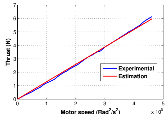
Fig. 9. Estimation and experimental of the thrust force relative to the square of motor velocity
