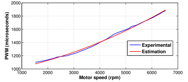
Fig. 7. Measured and approximated PWM signal and motor speed characteristics
