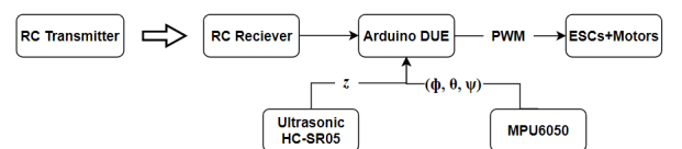
Fig. 5. Sunbird quadrotor prototype architecture
