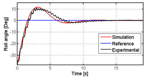
Fig. 13. Comparison of simulated and experimental roll angle step response with (k_p = 0.35, k_i = 0.28, k_d = 0.46)
